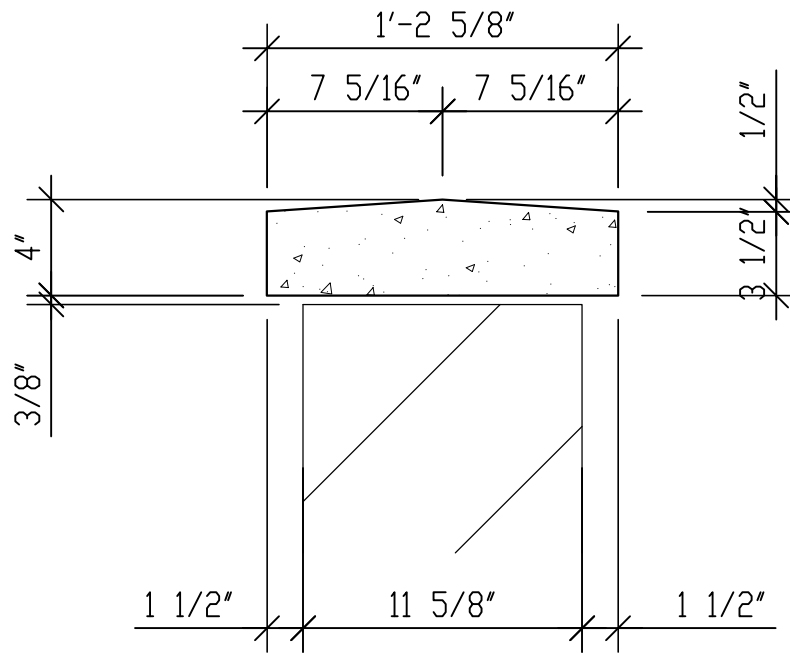
SECTION 1 1/2" = 1'-0"
