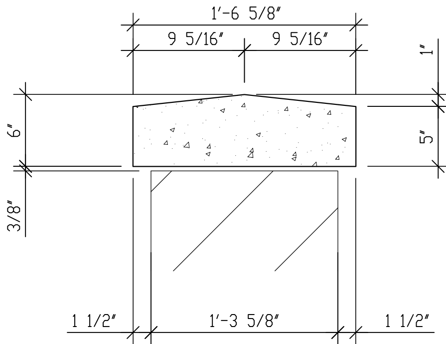
SECTION 1 1/2" = 1'-0"
