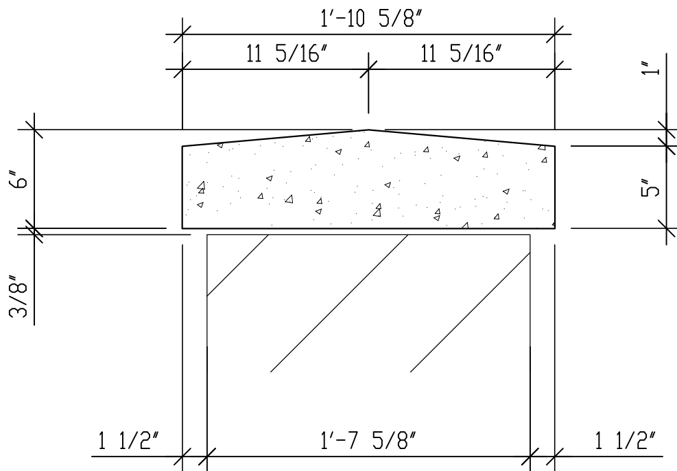
SECTION 1 1/2" = 1'-0"
