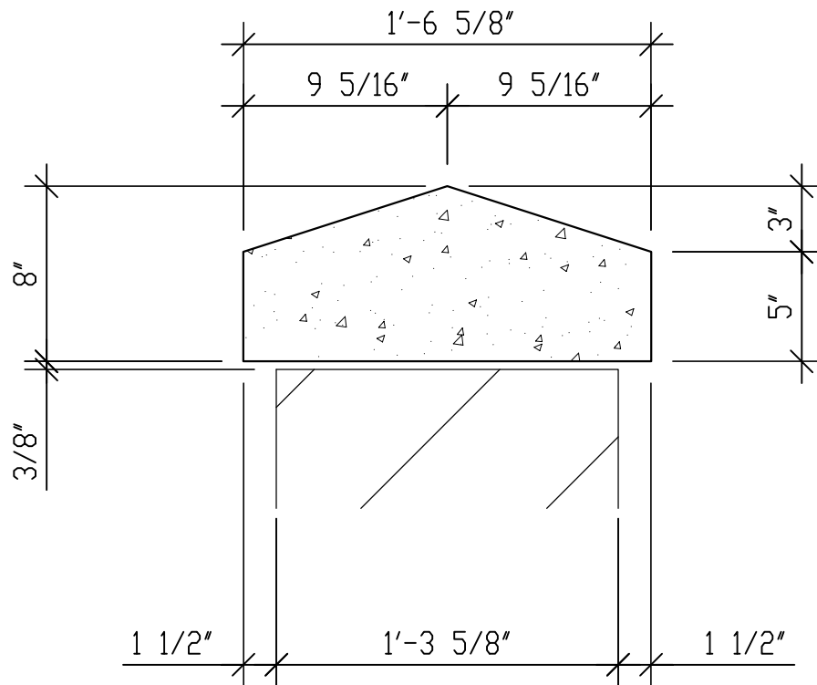
SECTION 1 1/2" = 1'-0"
