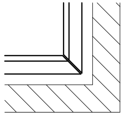
INSIDE MITER JOINT PLAN VIEW
