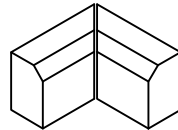
INSIDE MITER JOINT ISOMETRIC VIEW
