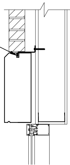
SECTION B/BB
