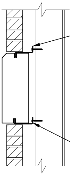
SECTION A/AA
