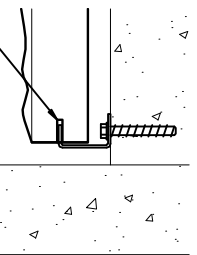
DETAIL D/D
