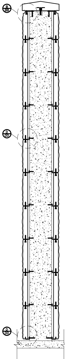
SECTION A/A
