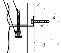
DETAIL C/C
