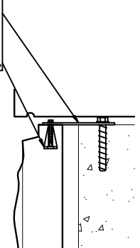
DETAIL B/B
