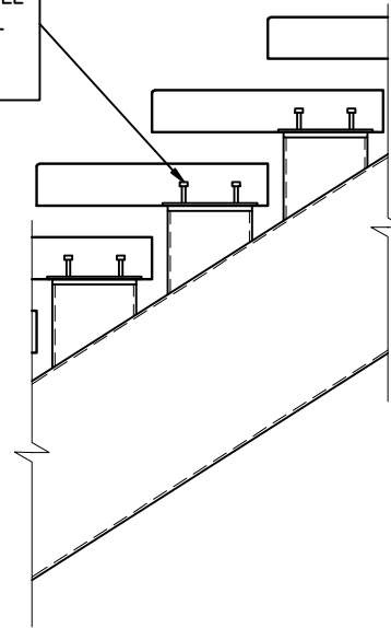
SECTION A/A
