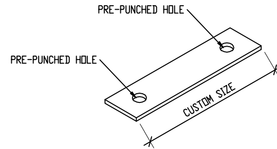
STRAP ANCHOR
