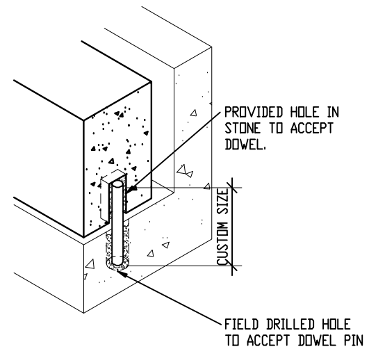
DOWEL PIN
