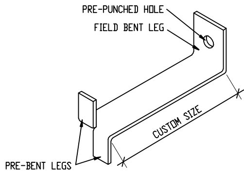
SPLIT-TAIL ANCHOR
