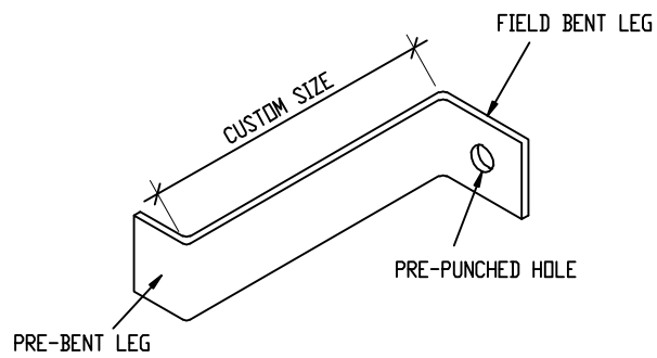
SIDE ANCHOR
