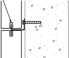
DETAIL C/CC
