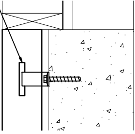
DETAIL B/BB
