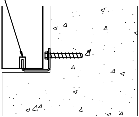
DETAIL D/DD
