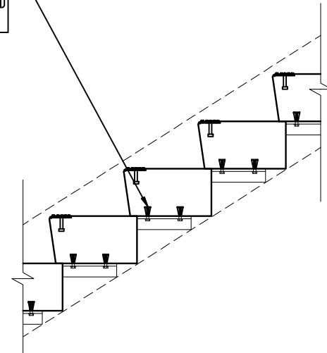
SECTION A/A
