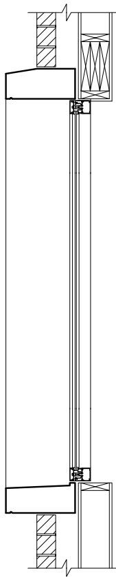
SECTION A/A
