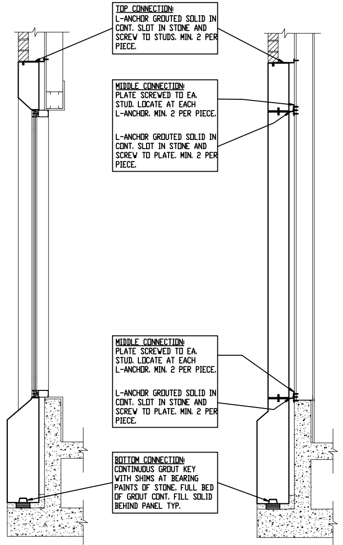
SECTION A/AA
